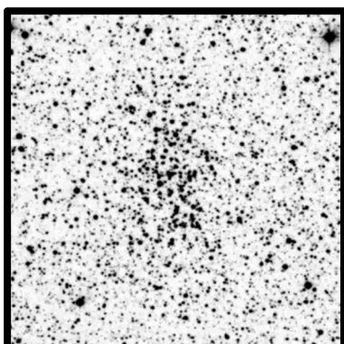
NGC 6802 10'
