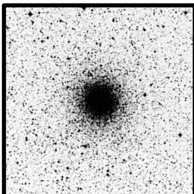
NGC 6356 10'
