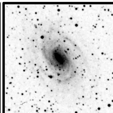
NGC 6384 19'
