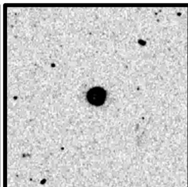
NGC 6369 "Little Ghost" 5'
