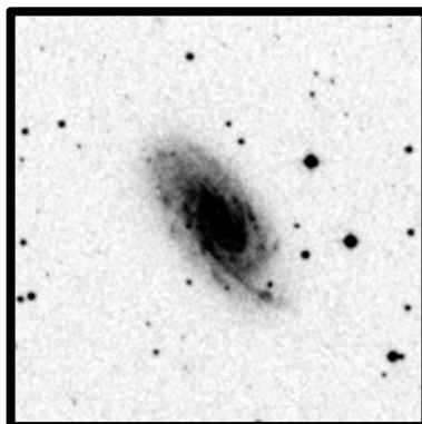
NGC 6643 6'
