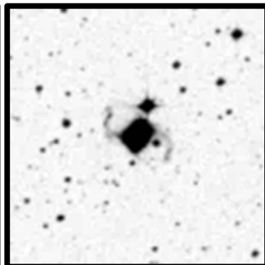
NGC 6309, "Box" 3'
