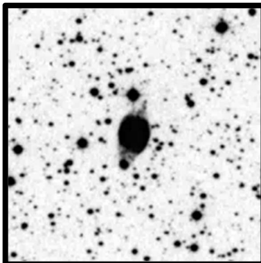
NGC6905, "Blue Flash" 5'
