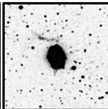
Ngc40, "Bow Tie" 5'
