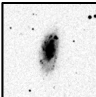
NGC7448, Arp 13 4'
