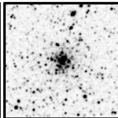
NGC 6642 5'
