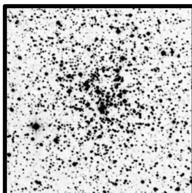
NGC 6819 10'
