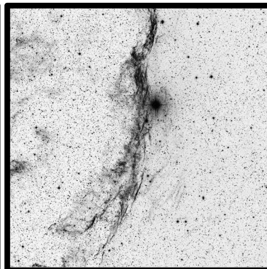
NGC6960, "Veil" 60'
