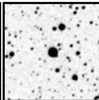
IC1747 3'
