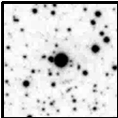
NGC6891 3'
