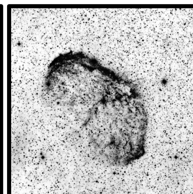
NGC 6888, "Crescent" 25'
