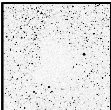
Barnard 68 10'
